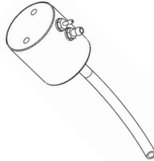
Capsule For Water Bottle
