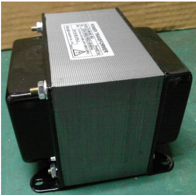
Linear Transformer 220V, 50/60Hz, 12V/6.8A, 24V//3A
